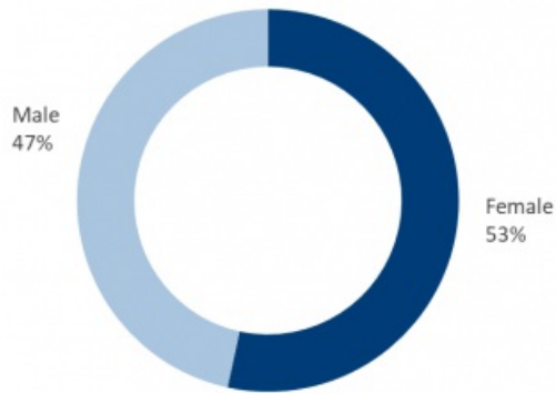
Percent of total COVID-19 case-patients by gender Wisconsin Electronic Disease Surveillance System, March 30, 2020 (n=1,221)
